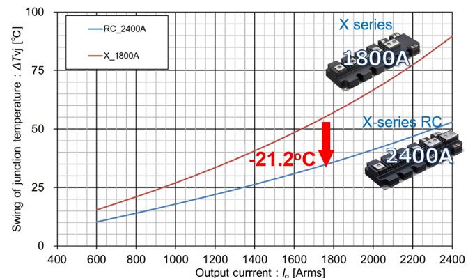
Figure 3: Calculation conditions: I_o=Vari. , f_c=3\text{ kHz} , f_o=1\text{ Hz} , V_{cc}=600\text{ V} , pf=0.9 , m=0.01 , nominal R_G , R_{th(s-a)}=6\text{ K/kW} , R_{th(c-s)}=1.4\text{ K/kW} (with 3 W thermal grease), T_a=50\text{ °C}
