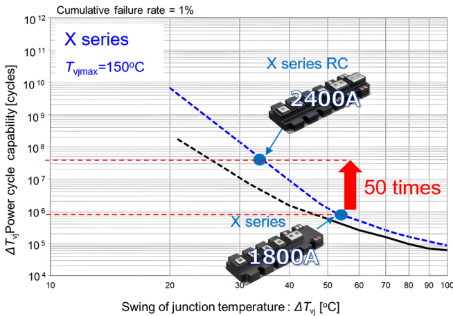
Figure 4: 1200V PrimePACK™3+ ΔTvj Power cycle lifetime comparison I o =1800Arms
