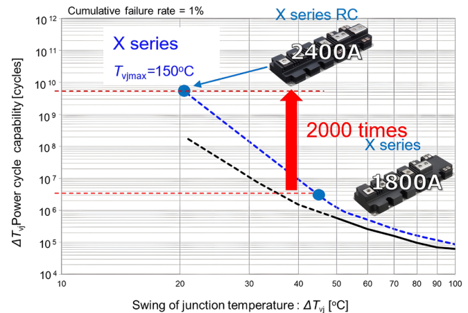
Figure 6: 1700V PrimePACK™3+ ΔTvj Power cycle life
