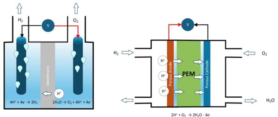
Figure 1: Electrolysis Cell vs Fuel Cell Schematic
