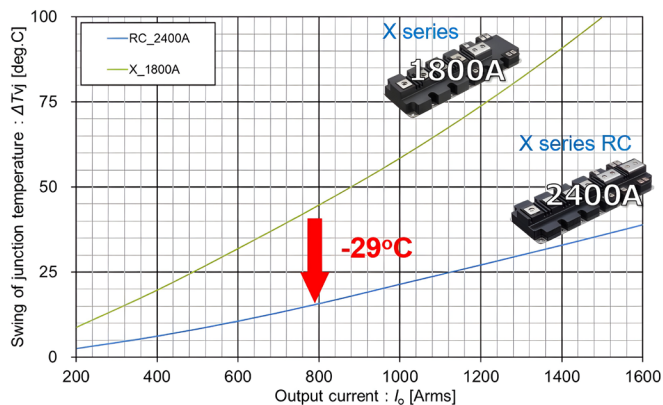
Figure 5: Calculation conditions: I o =Vari., fc=3kHz, fo=5Hz, Vcc=1200V, pf=-0.9, m=1, Standard RG, Rth(s-a)=4.7°C/kW, Rth(c-s)=1.4°C/kW (with 3W thermal grease), Ta=35°C
