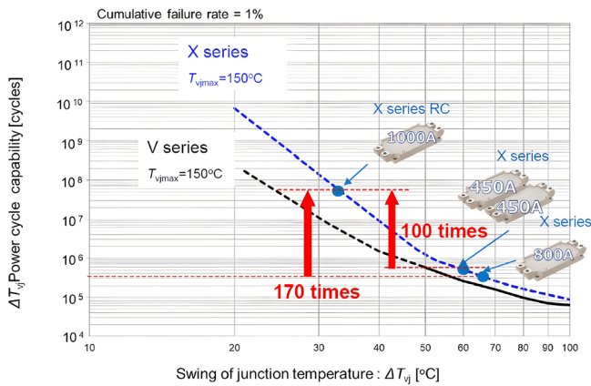
Figure 8: 1200V DualXT \Delta T_{vj} Power cycle life comparison
